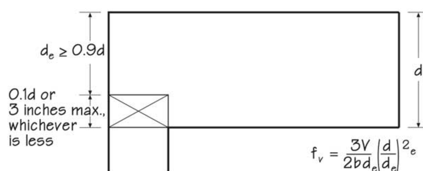
(f) Tension-side Notch
