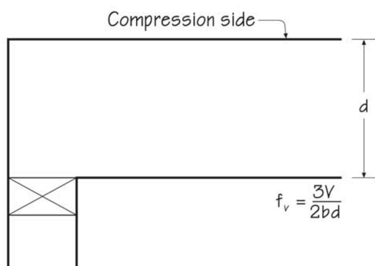
(a) Square End Bearing
