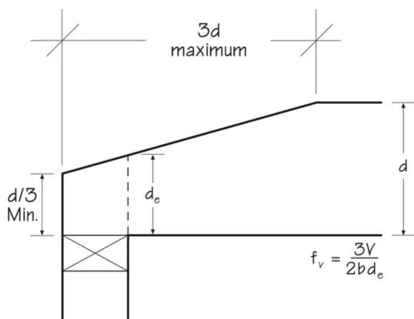
(c) Sloped End Cut for Roof Drainage
