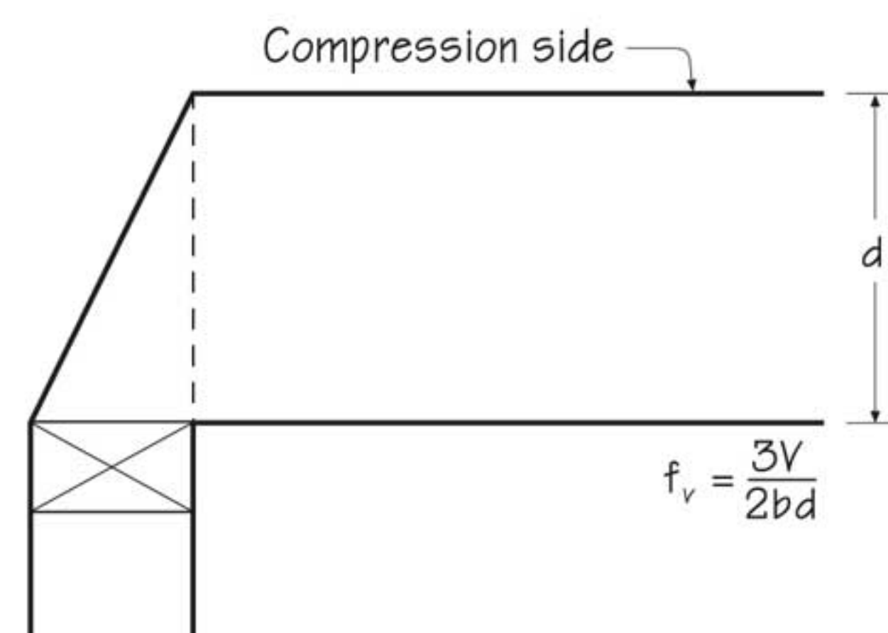
(b) Slope End Bearing
