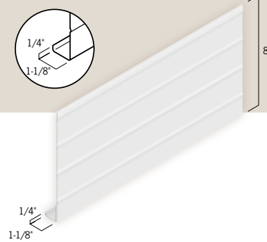
4", 6", 8" and 10" Ribbed Aluminum Fascia (0495, 0480, 0481, 0535)
