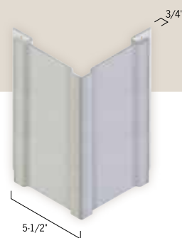
6" Traditional Corner Post (1250)
