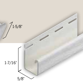
5/8" J Trim (1035)
