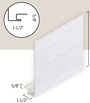
8" Vinyl Fascia (0490)
