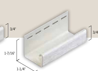
1 1/4" J Trim (1045)
