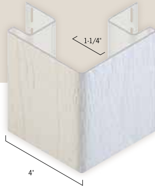
4" Outside Corner Post (1104)
