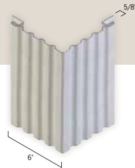
6" Designer Corner Post (1107)
