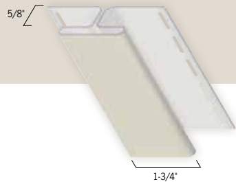
H Trim (1179)
