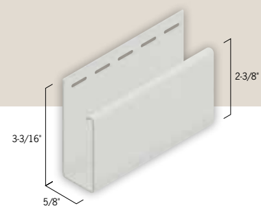
Super J Trim (1056)
