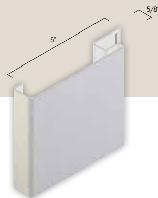
5" Window Surround (1055)
