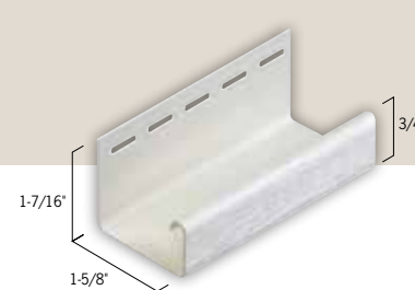
1 5/8" J Channel (1059)
