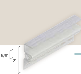
Frieze Trim (VTFBR)
