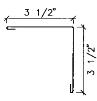
Corner Cap
