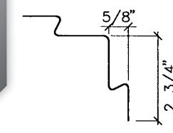
Base Corner Vinyl
