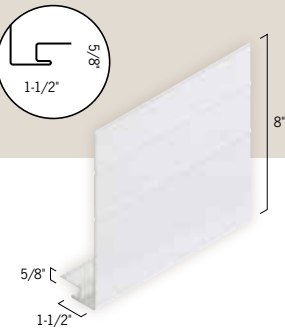
8" Vinyl Fascia (0490)
