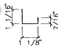
J Channel 1 1/8"
