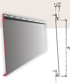
Smooth Horizontal 8"
